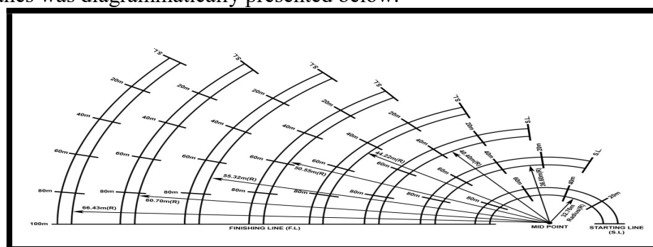
Fig.-1: Layout of Different Eight (8) Curve Lanes of 100m Distance
